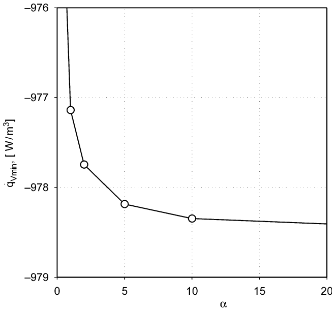
Fig. 23. Additional heat source \dot{q}_{V,min} vs. \alpha , entropy minimization.
