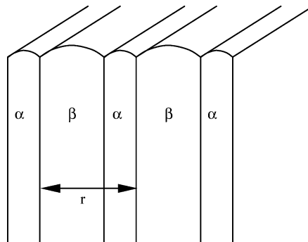
Fig. 2. Schematic of the eutectic solidification.
