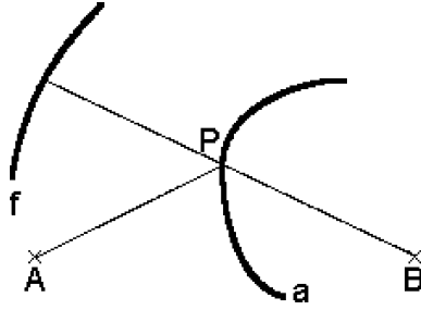
Fig. 4. Reflection by an aplanatic mirror surface (real-virtual case).
