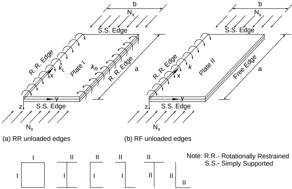
Fig. 1. Geometry of orthotropic plate elements in FRP shapes.
