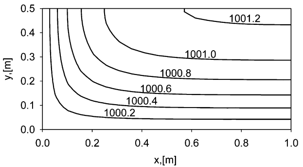
Fig. 17. Temperature [K], entropy minimization, \alpha = k_y/k_x = 5.0 (anisotropic solid).
