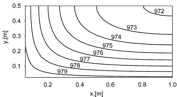
Fig. 15. Joule heat-generation rate [\text{W}/\text{m}^3] , entropy minimization, \alpha = k_y/k_x = 1.0 (isotropic solid).
