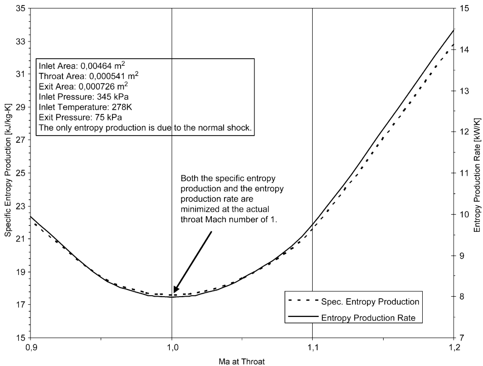
Fig. 7. Entropy production of normal shock in a converging–diverging nozzle.
