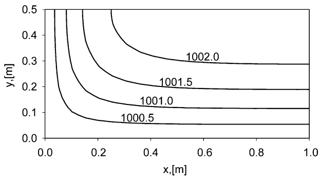
Fig. 16. Temperature [K], classical problem, \alpha = k_y/k_x = 5.0 (anisotropic solid).
