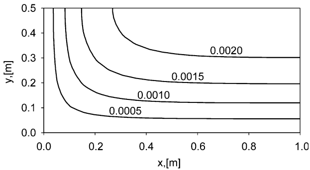
Fig. 18. Entropy source [W/m 3 K], classical problem, \alpha = k_y/k_x = 5.0 (anisotropic solid).
