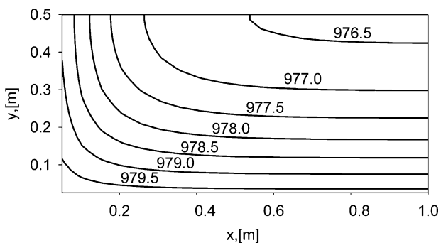
Fig. 20. Joule heat-generation rate [ \text{W/m}^3 ], classical problem, \alpha = k_y/k_x = 5.0 (anisotropic solid).
