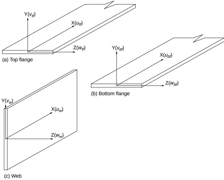
Fig. 3. Coordinate system of I- or C-beam.
