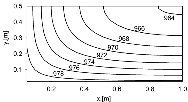
Fig. 14. Joule heat-generation rate [\text{W}/\text{m}^3] , classical problem, \alpha = k_y/k_x = 1.0 (isotropic solid).
