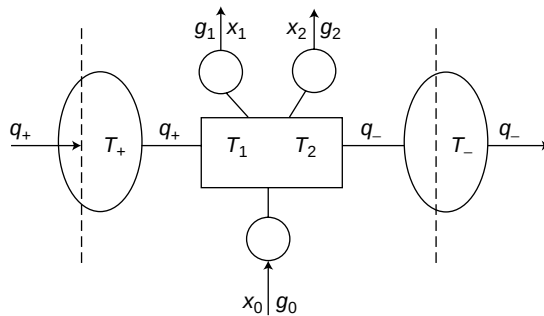
Fig. 3. Thermal separation system.
