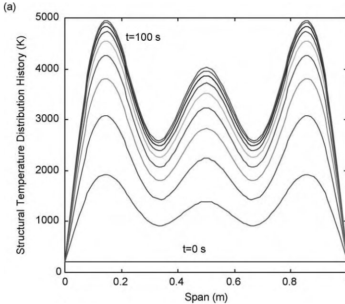
Fig. 2. (a) Boundary layer heating of flat panel at Mach 10. (No piston-theory heating, C_{TAE} = 0 ). (b)–(f) Elastothermoelectric control of aerodynamic heating via vibrating aerothermoelastic panel at Mach 10, C_{TAE} = 100 .
