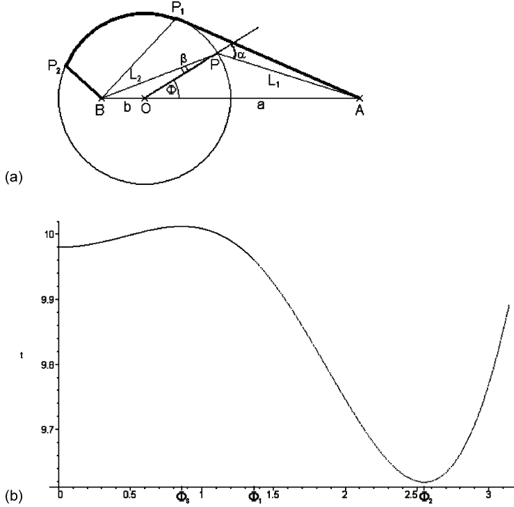
Fig. 2. (a) Circular refracting curve. (b) Angle–propagation time relationship (parameter values: a = 5 , b = 0.3 , v_1 = 4.6 , v_2 = 1 ).
