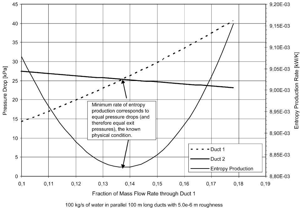
Fig. 4. Pressure drop and entropy production in two-duct system.
