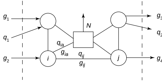
Fig. 1. Open thermodynamic system with transformer.
