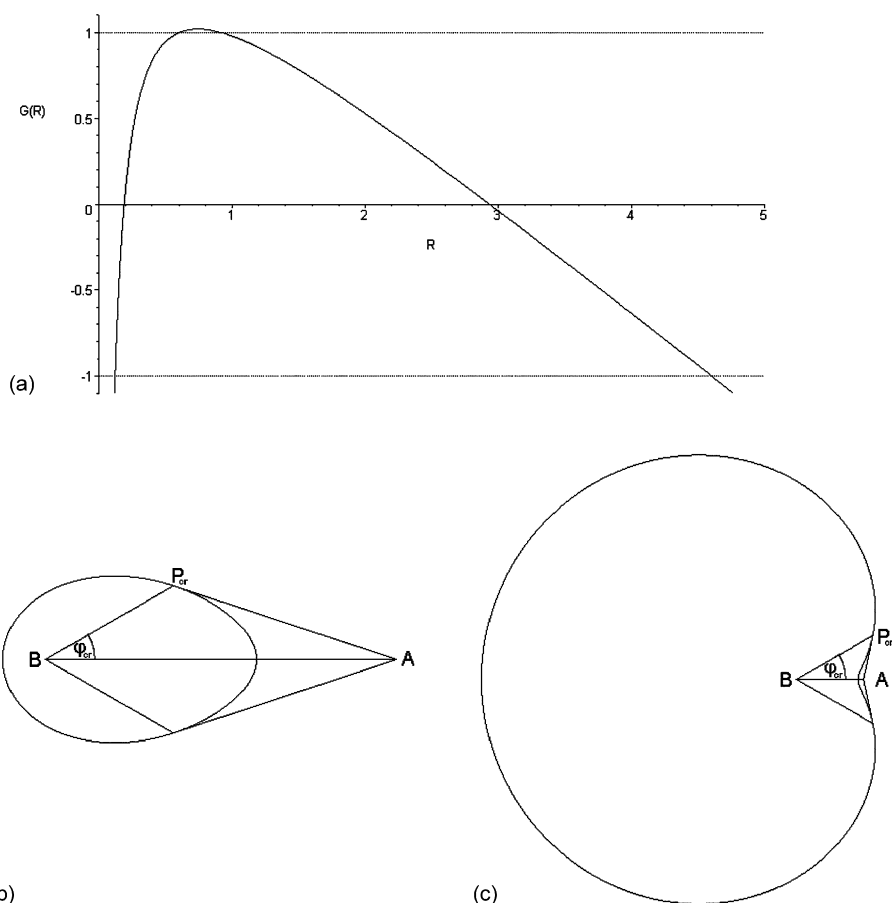
Fig. 6. Case (iii), n = 1.5 , E = 1.3 , d = 1 , v_A = 1 , v_B = 1/n (a) The graph of G(r) . (b) Real–real image formation. (c) Real–virtual aplanatic curve.
