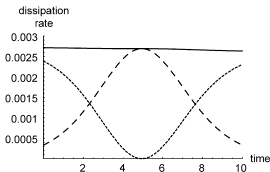
Fig. 8. Nonlinear example. Dissipation rate along the optimal trajectory for the slow case t_f = 10 . The values of the other parameters for this example were: k_{AA} = k_{BB} = 1 , a = 10 . Compare this to Fig. 6: The variations of the dissipation rate along the trajectory are much smaller. The dissipation rate is lower roughly by a factor 100, the square of the increase in available time.
