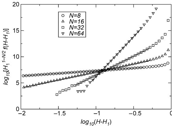
Fig. 1. Logarithmic plot of the rescaled distribution H_1^{1-N/2} f(H - H_1) as a function of the transformed variable H - H_1 for N = 8 (circles), 16 (triangles up), 32 (squares), and 64 (triangles down) anharmonic oscillators. The solid straight lines are the best fit to the simulation data of the expected power-law behavior (Eq. (79)). The slopes are 1.0068 (1.0), 3.07 (3.0), 7.21 (7.0) and 15.27 (15.0) for N = 8, 16, 32 and 64 , respectively. The numbers in parentheses indicate the expected values obtained from Eq. (80). The departure from the power-law behavior at the extremes of the curves is due to finite-time sampling.
