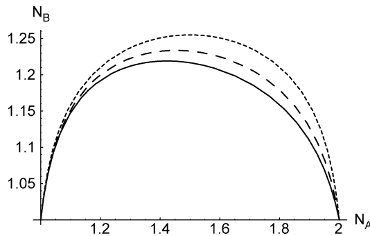
Fig. 7. Nonlinear example. The optimal path in the 2D space of the extensive parameters N_A and N_B for an available time t_f = 1 (solid line), t_f = 10 (dashed line) and for the limit t_f \rightarrow \infty (dotted line, identical to Fig. 3). The values of the other parameters were: k_{AA} = 1 , k_{BB} = 2 , a = 10 .
