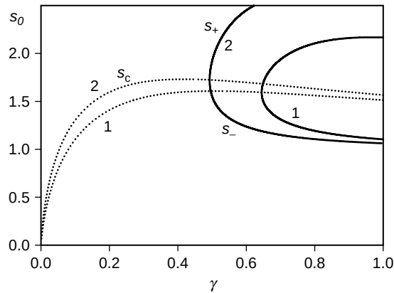
Fig. 2. Stationary value of the avalanche size s_0 vs. exponent \gamma at \sigma^2 = 100, 150 (curves 1 and 2 correspondingly).
