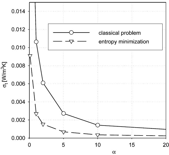
Fig. 22. Entropy generation \sigma_t vs. \alpha = k_y/k_x .
