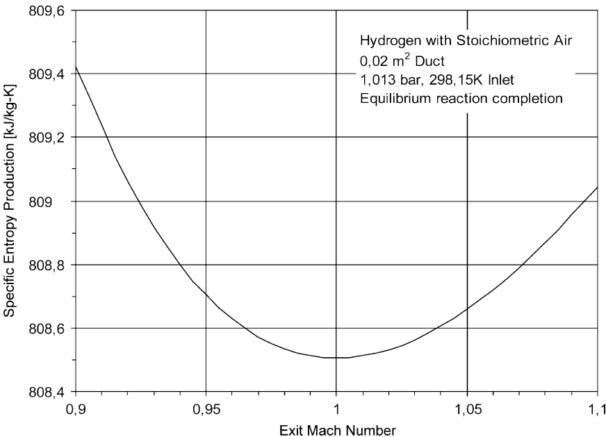
Fig. 10. Specific entropy production in Chapman–Jouget detonation versus exit Mach number.
