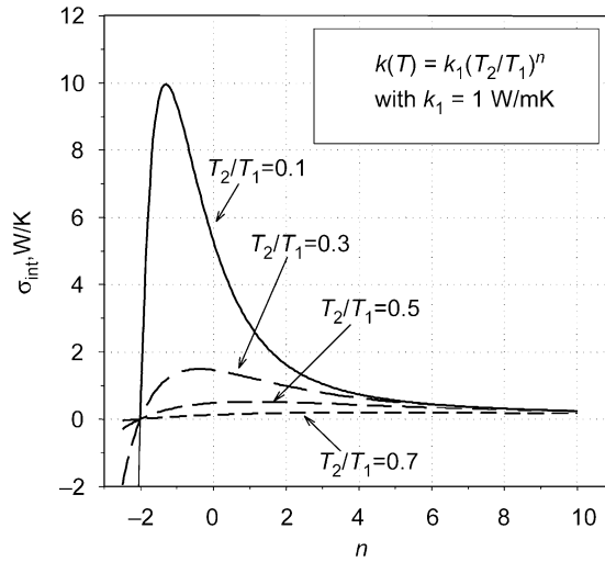
Fig. 4. Internal entropy-generation rate \sigma_{\text{int}} vs. n for different T_2/T_1 .
