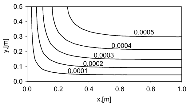
Fig. 19. Entropy source [ \text{W/m}^3 \text{ K} ], entropy minimization, \alpha = k_y/k_x = 5.0 (anisotropic solid).
