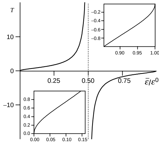
Fig. 1. The energy dependencies of the avalanche-ensemble temperatures: nonstationary magnitude T vs. ratio \bar{\mathcal{E}}/\mathcal{E}^0 .
