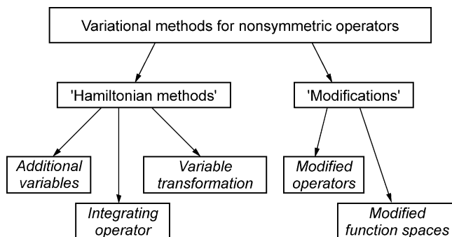
Fig. 1. Possible routes to construct a variational principle.
