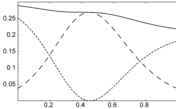
Fig. 6. Nonlinear example. Total dissipation rate along the optimal trajectory solid curve. Dashed curve relates to substance A, dotted curve to substance B only. Since the driving forces are not linear in the fluxes, the total dissipation rate is not constant along the path. The values of the parameters for this example were: k_{AA} = 1 , k_{BB} = 2 , a = 10 , t_f = 1 .
