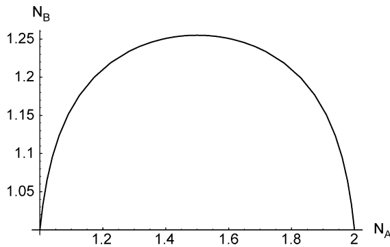
Fig. 3. Linear example. The optimal path in the 2D space of the extensive variables. The values of the parameters for this example were: k_{AA} = 1 , k_{BB} = 2 , a = 10 , t_f = 10 .
