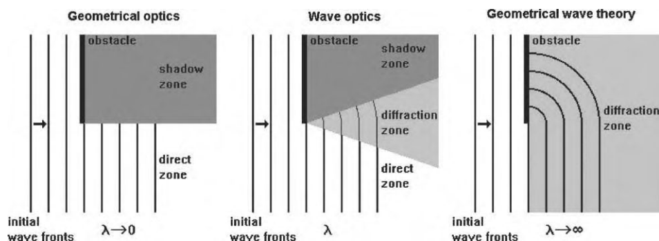
Fig. 1. Relation between geometrical optics, wave optics and geometrical wave theory.
