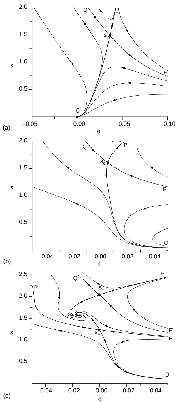
Fig. 4. Phase portraits of the system with white noise at \sigma^2 = 100 : (a) \gamma = 0.25 ; (b) \gamma = 0.6 ; (c) \gamma = 0.75 .
