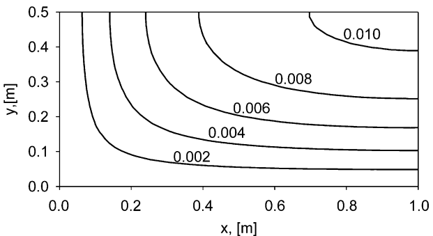
Fig. 12. Entropy source [W/m^3 K] , classical problem, \alpha = k_y/k_x = 1.0 (isotropic solid).
