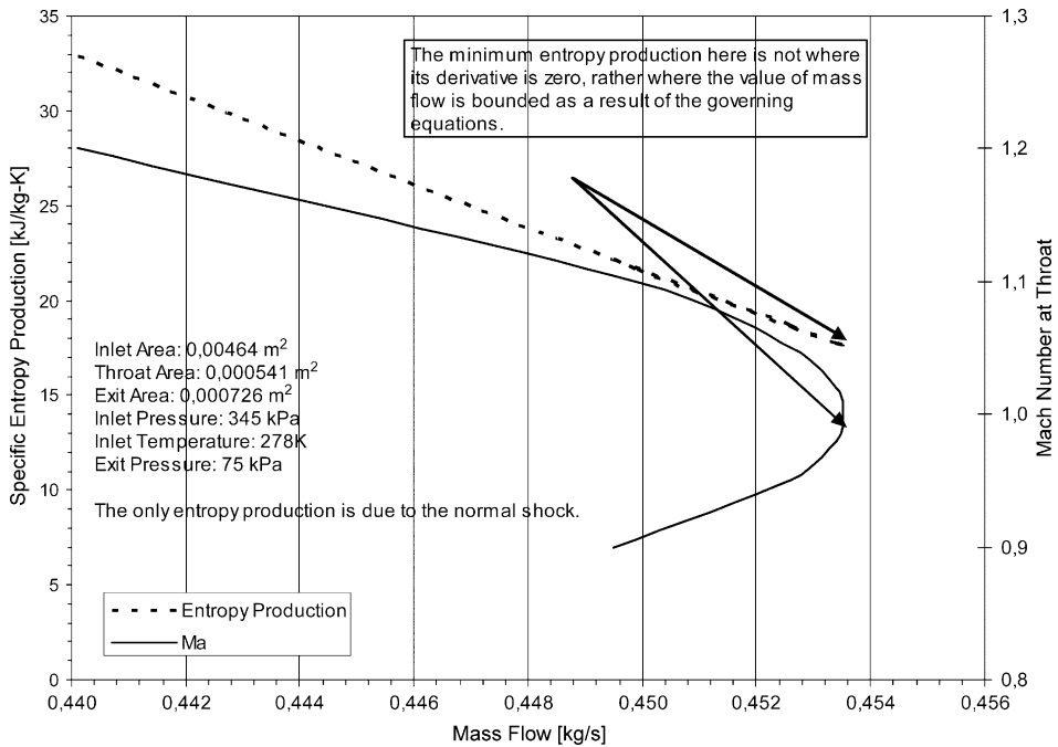
Fig. 8. Specific entropy production and throat Mach number for normal shock in a converging–diverging nozzle.
