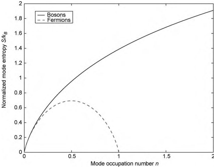
Fig. 1. Entropy S/k_B for a single field mode as a function of mean occupation number n : bosons (solid curve) and fermions (dashed curve). For fermions, 0 \leq n \leq 1 .
