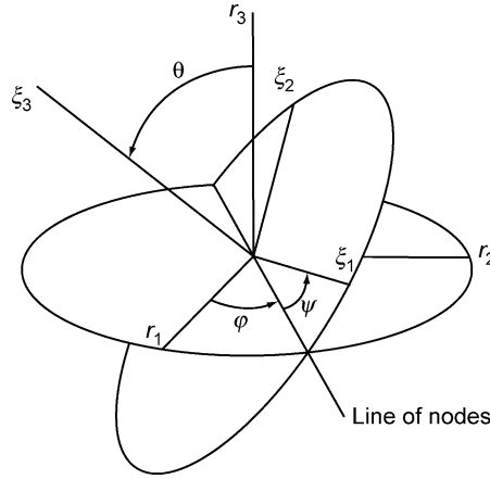
Fig. 1. The definition of the Euler angles for an arbitrary particle.
