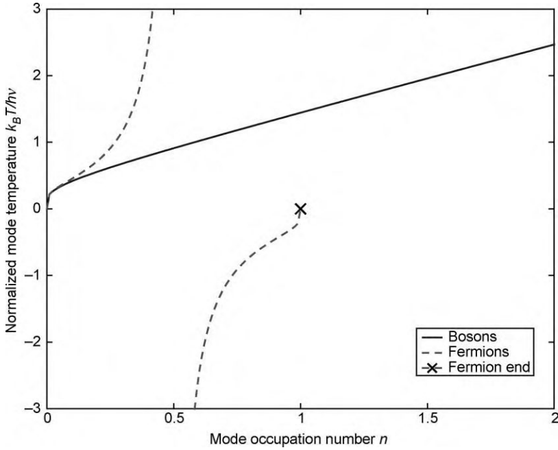
Fig. 2. Normalized temperature k_B T / h\nu for a single field mode of energy \epsilon = h\nu as a function of mean occupation number n : bosons (solid curve) and fermions (dashed curve). For fermions, 0 \leq n \leq 1 .
