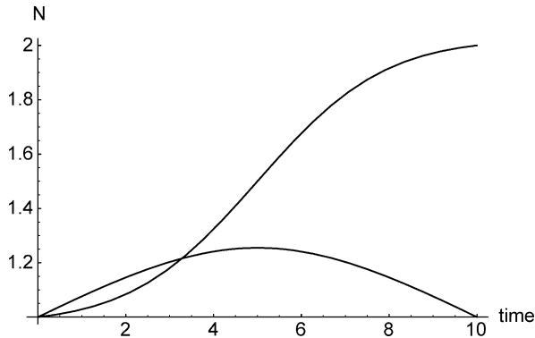
Fig. 1. Linear example. Time evolution of the concentrations of the two substances N_A , and N_B for the optimal trajectory. Note that along this trajectory some B is added and then removed. The values of the parameters for this example were: k_{AA} = 1 , k_{BB} = 2 , a = 10 , t_f = 10 .
