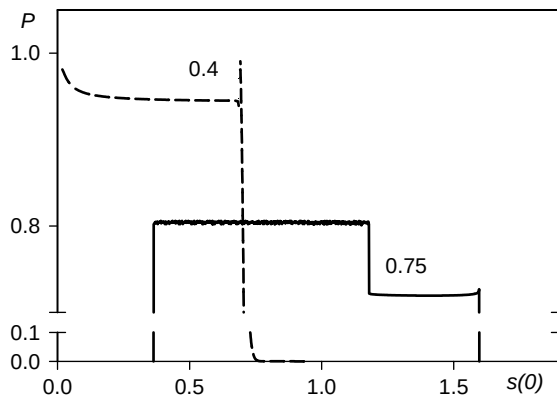
Fig. 5. Dependence of the probability P of realization of different trajectories on the initial value of the avalanche size s(0) at \sigma^2 = 100 (dashed and solid curves correspond to \gamma = 0.4, 0.75 . The initial value of the conjugate momentum is \phi(0) = 0.015 .
