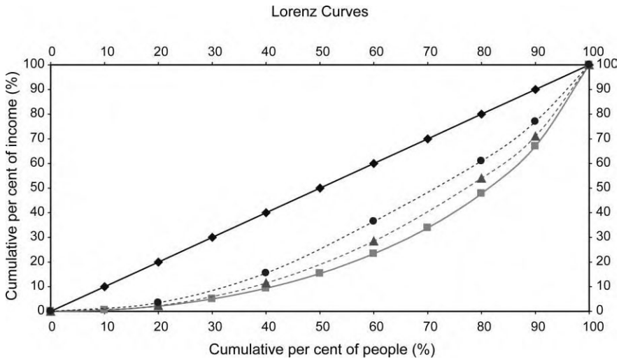
Fig. 2. Lorenz curves. Solid lines: the straight 45° line (Lorenz curve in the case of a completely egalitarian income distribution) and the Lorenz plot in the case of an exponential distribution. The Gini coefficient—the area between the two solid lines divided by the total area under the 45° line—is \frac{1}{2} (50%). Dashed lines: the Lorenz plots for Romania (●, 1991; ▲, 1997). Source: http://www.wider.unu.edu/wiid/wwwiid.htm .
