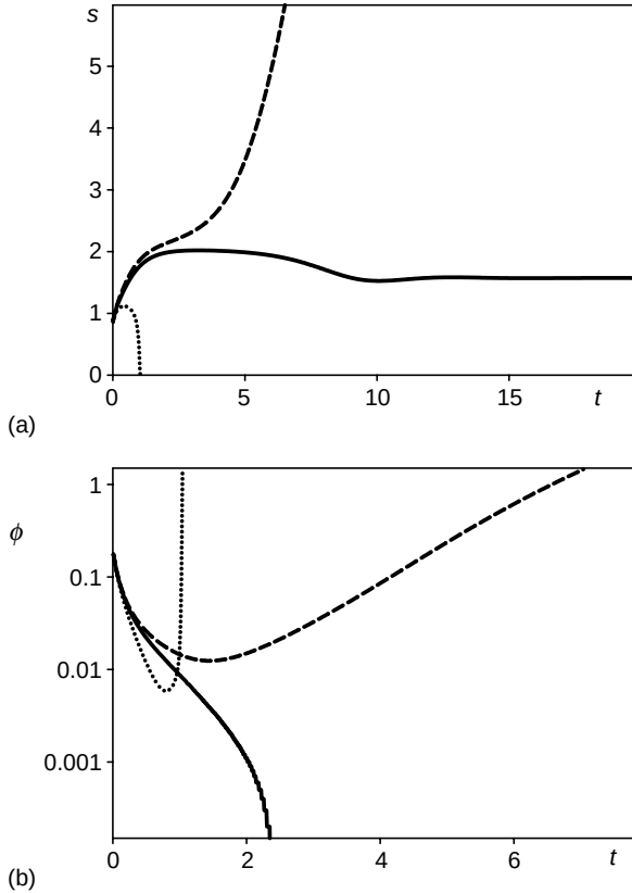
Fig. 6. A typical appearance of the temporal behavior for: (a) the avalanche size; (b) the conjugate momentum at \gamma = 3/4 , \sigma^2 = 100 (solid curves correspond to the trajectories inside the domain FS_cF' , dashed lines correspond to trajectories above the separatrix F'S_+ , dotted curves correspond to domain of small values s(0) ).
