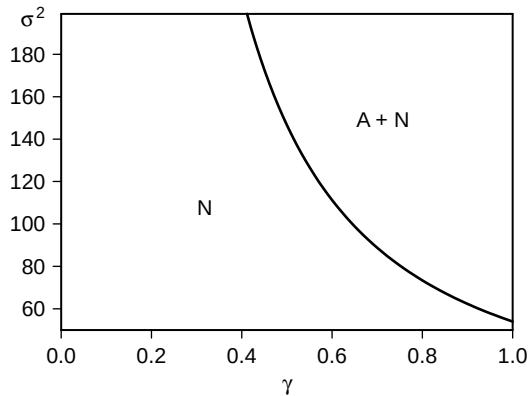
Fig. 3. Phase diagram of stationary avalanche formation.
