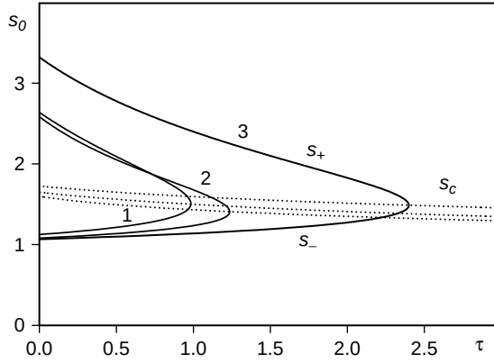
Fig. 8. Stationary solutions for the system with colored noise: 1 - \sigma^2 = 150 , \gamma = 0.75 ; 2 - \sigma^2 = 150 , \gamma = 0.9 ; 3 - \sigma^2 = 200 , \gamma = 0.75 .
