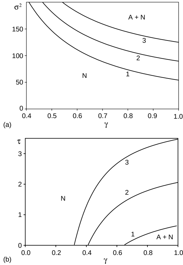
Fig. 7. Phase diagrams for the system with colored noise: (a) \sigma^2 vs. \gamma curves 1, 2, 3 corresponds to \tau = 0.001, 0.5, 1 ; (b) \tau vs. \gamma at \sigma^2 = 100, 200, 300 (curves 1, 2, 3).
