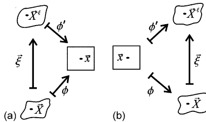
Fig. 3. Two possible approaches for comparison of the excited motion superimposed on a normal motion of fluid element.
