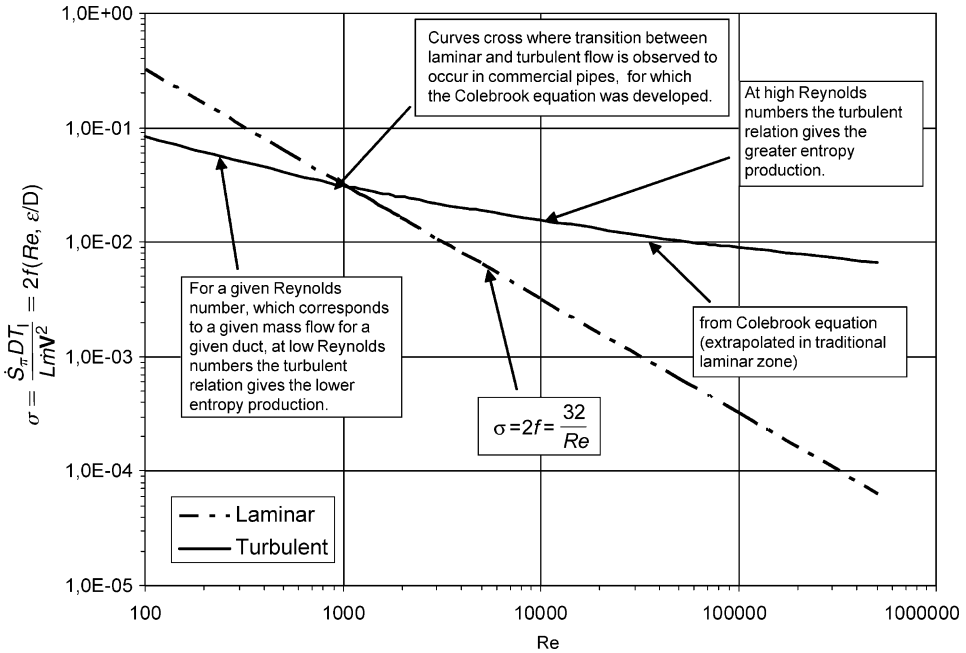
Fig. 1. Dimensionless entropy production \sigma versus Reynolds number Re for adiabatic, incompressible flow in long, smooth ducts.
