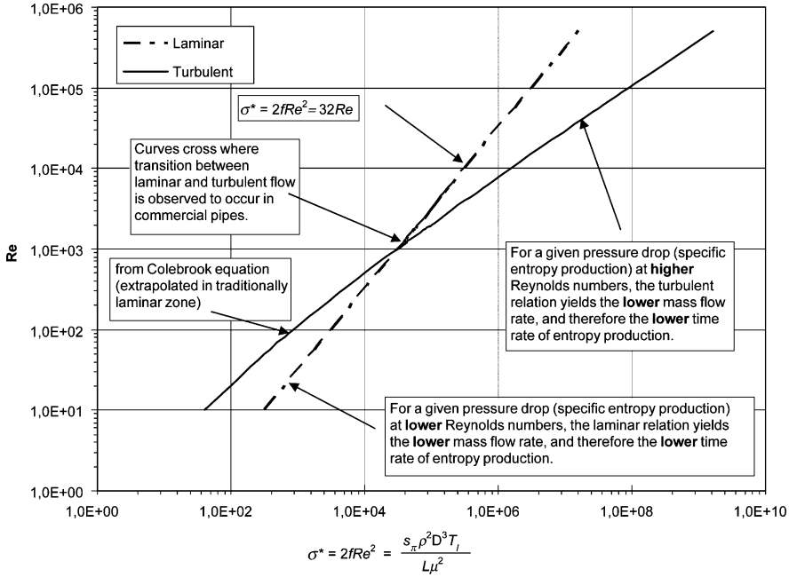
Fig. 2. Reynolds number versus dimensionless entropy production, \sigma^* for adiabatic, incompressible flow in long, smooth ducts.
