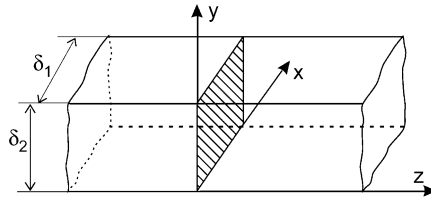
Fig. 9. Infinite-rod geometry.
