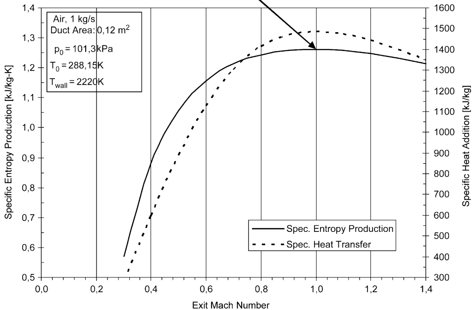
Fig. 6. Rayleigh flow example.
