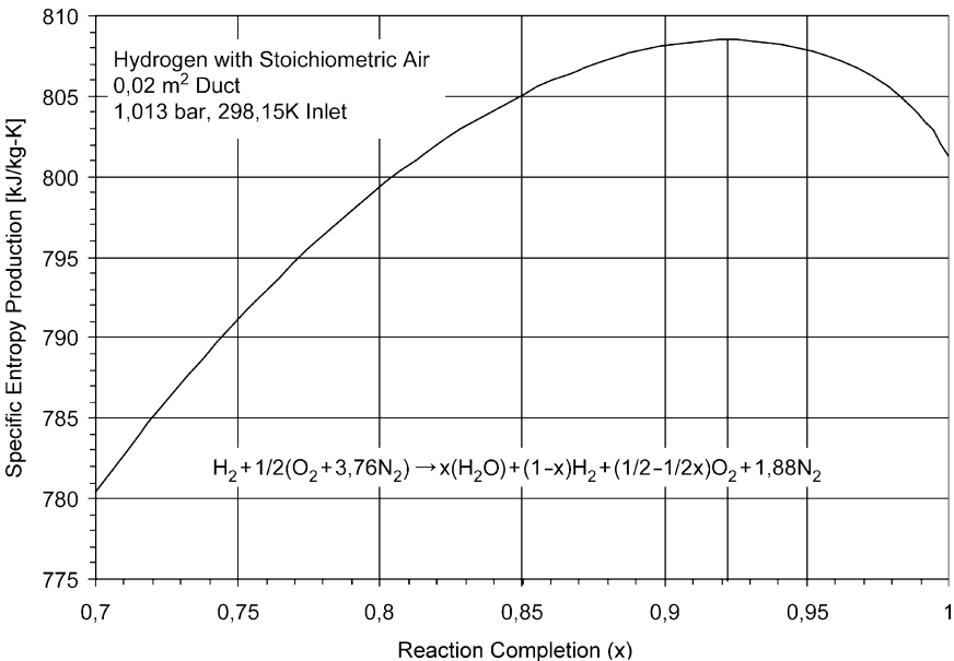
Fig. 9. Specific entropy production in Chapman–Jouget detonation versus reaction completion.
