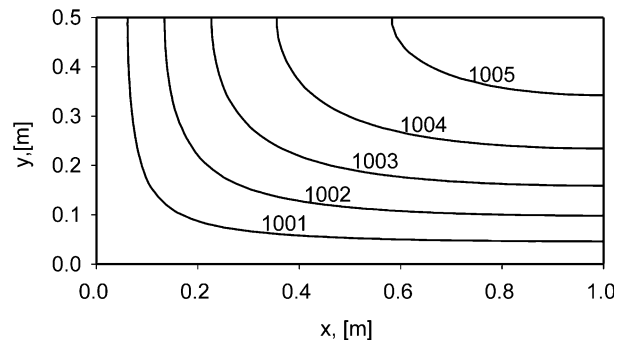
Fig. 11. Temperature [K], entropy minimization, \alpha = k_y/k_x = 1.0 (isotropic solid).
