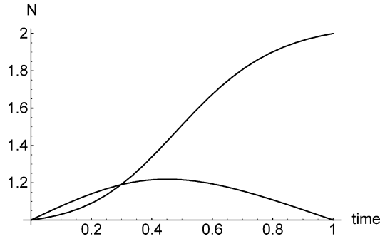
Fig. 4. Nonlinear example. Time evolution of the concentration of the two substances for the optimal trajectory. Note that along this trajectory some B is added and then removed. The values of the parameters for this example were: k_{AA} = 1 , k_{BB} = 1 , a = 10 , t_f = 1 .
