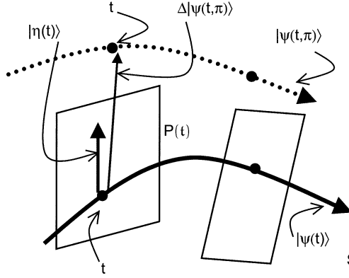
Fig. 1. Accompanying tangent or perturbation space P(t) along the trajectory |\psi(t)\rangle of the process in state space S . Perturbation: \Delta|\psi(t; \pi)\rangle , representative: |\eta(t)\rangle , being approximately parallel to \Delta|\psi(t; \pi)\rangle .
