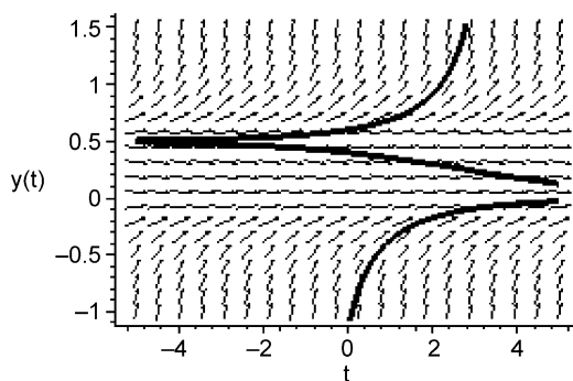
Fig. 4. The solutions of Eq. (26) for \alpha = 2 ; s = 1 ; \lambda = 0.5 . The asymptotic behavior of solutions is extremely sensitive to the initial conditions. The system can evolve following one of the two asymptotic solutions or can shift from one to another.
