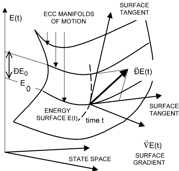
Fig. 1. Evolutionary energy \bar{D}E(t) : energy-conservation-compliant (ECC) directional change in energy process on the energy surface E(t) .
