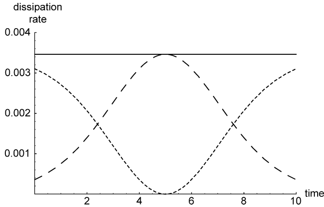
Fig. 2. Linear example. Dissipation rate along the optimal trajectory. Total dissipation (solid curve) is constant along the optimal trajectory, dashed curve refers to the flux of A, dotted curve to the flux of B. The values of the parameters for this example were: k_{AA} = 1 , k_{BB} = 2 , a = 10 , t_f = 10 .
