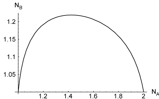
Fig. 5. Nonlinear example. The optimal path in the 2D space of the concentrations. The values of the parameters for this example were: k_{AA} = 1 , k_{BB} = 1 , a = 10 , t_f = 1 .
