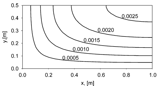
Fig. 13. Entropy source [\text{W}/\text{m}^3 \text{ K}] , entropy minimization, \alpha = k_y/k_x = 1.0 (isotropic solid).
