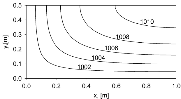
Fig. 10. Temperature [K], classical problem, \alpha = k_y/k_x = 1.0 (isotropic solid).
