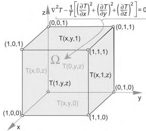
Fig. 7. 3D boundary-value problem.
