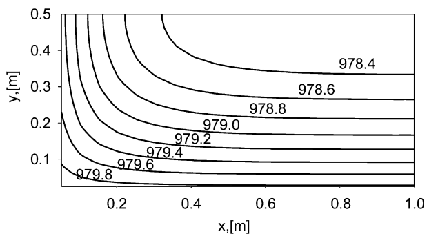
Fig. 21. Joule heat-generation rate [ \text{W/m}^3 ], entropy minimization, \alpha = k_y/k_x = 5.0 (anisotropic solid).
