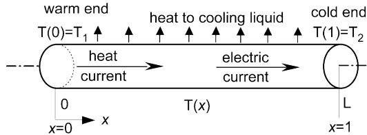
Fig. 8. Electric power cable.
