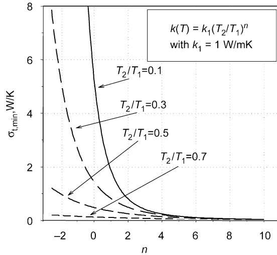
Fig. 5. Global entropy-generation rate (Eq. (13)) vs. n and T_2/T_1 .
