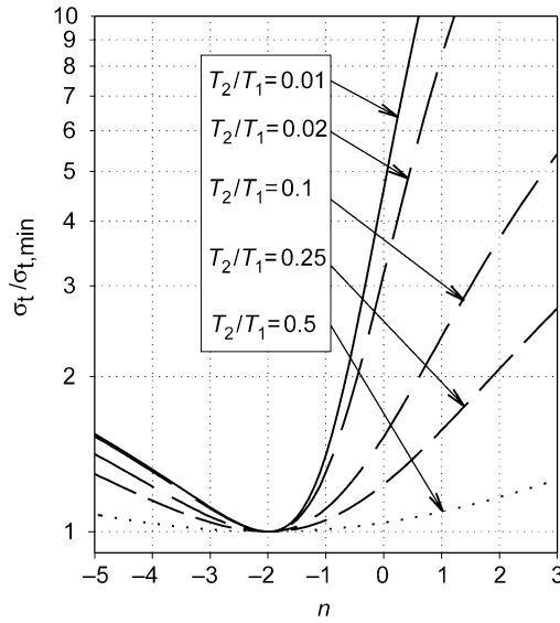
Fig. 2. N vs. n for different T_2/T_1 .
