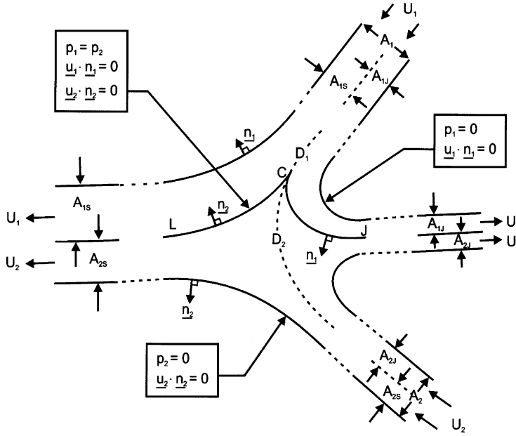
Fig. 1. The potential flow field describing the two impinging streams consists of two regions D_1 and D_2 . The upper first incoming stream is the stronger of the two, having a higher Bernoulli constant. The cusp point C is a stagnation point for the flow in D_2 . The streamlines CJ and CL are contact discontinuities on which the normal components of the velocity fields in each region vanish and the pressures in each region are equal.
