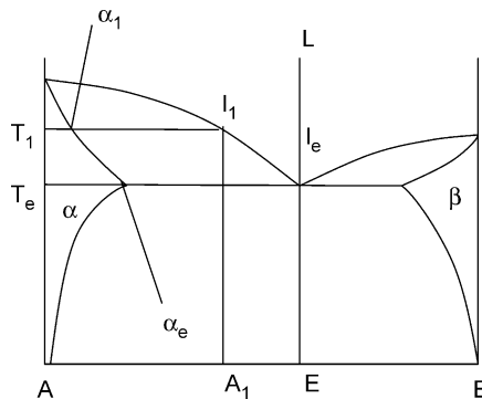
Fig. 1. Phase diagram showing eutectic solidification of liquid L.
