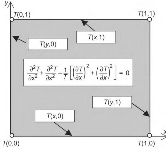
Fig. 6. General scheme of 2D boundary-value problem with first-kind boundary conditions.
