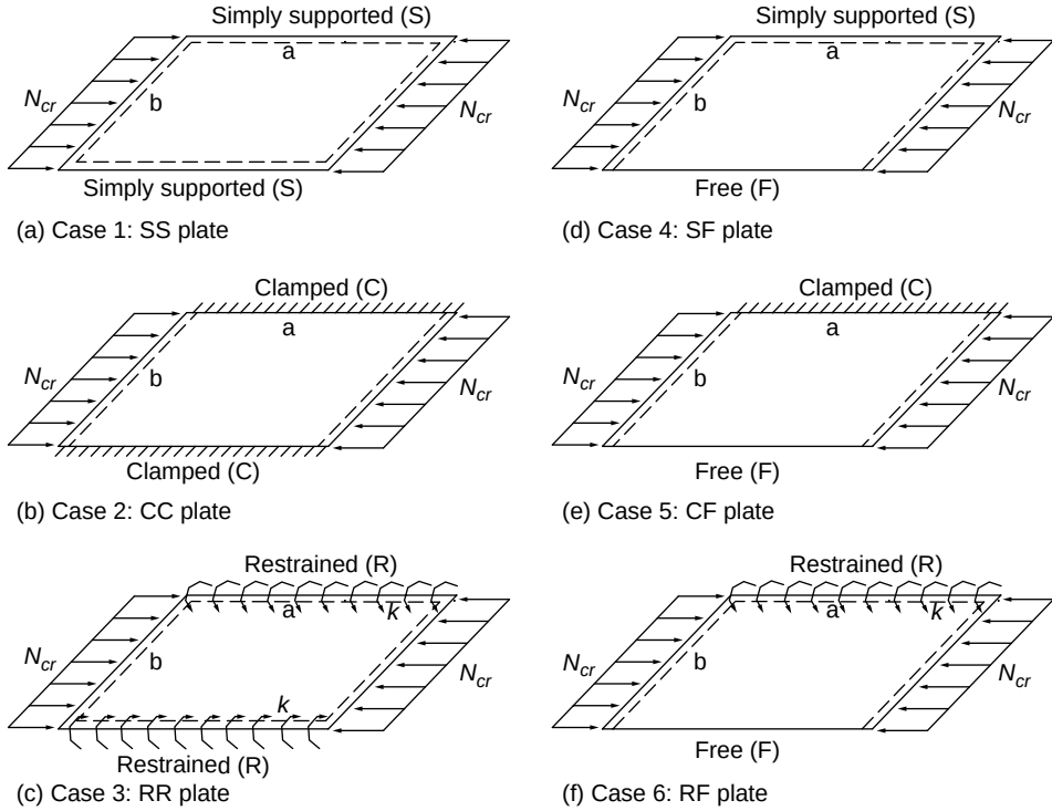
Fig. 2. Common plates with various unloaded edge conditions.
