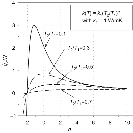
Fig. 3. \dot{q}_V vs. n for different T_2/T_1 .
