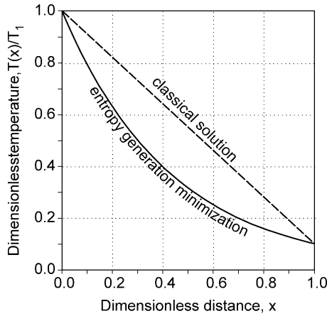
Fig. 1. Temperature distributions in the plane wall.
